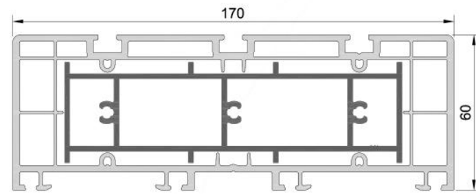
1701 Hebe-Schiebe Frame Profile
