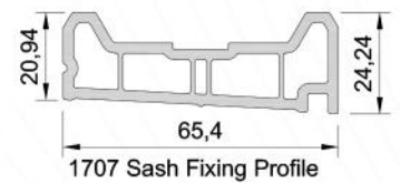
1707 Sash Fixing Profile
