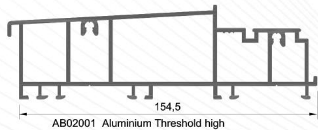
AB02001 Aluminium Threshold high
