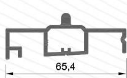
AB02002 Outer Rail
