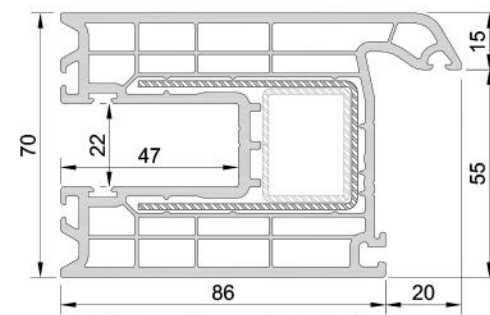
1702 Hebe-Schiebe Sash Profile
