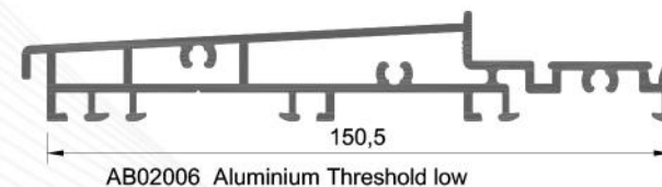
AB02006 Aluminium Threshold low
